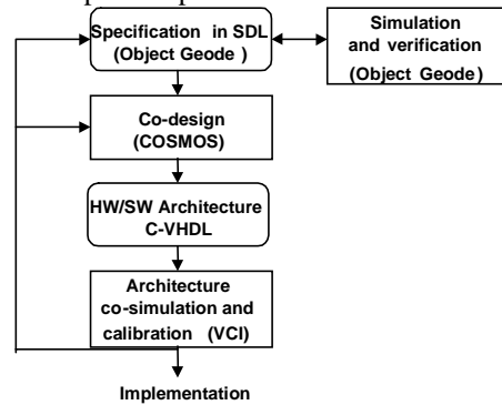
Fig. 5: Design flow adopted for the architecture exploration of the NIC system.
