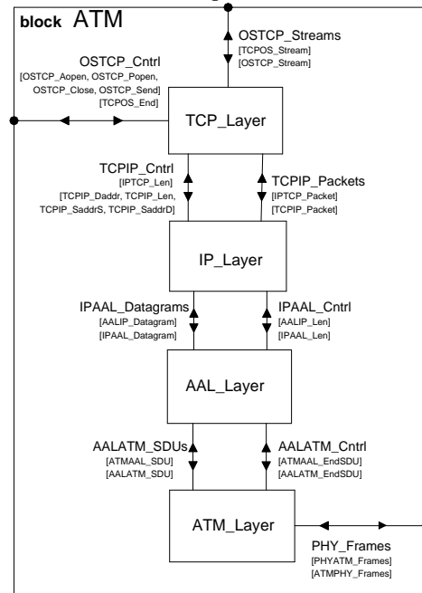
Fig. 3: Structure of the NIC system described in SDL.
