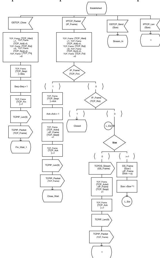
Fig. 4: Extract of the behavioral description of the TCP layer.
