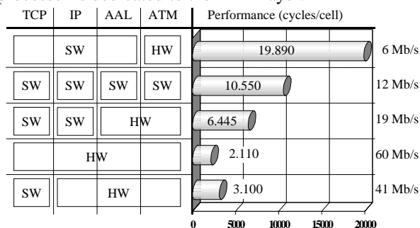
Fig. 6: Performance of different ATM NIC implementations.
